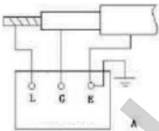
Test cablu
